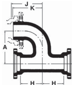
MJ Hydrant Tee Anchoing on the Branch
