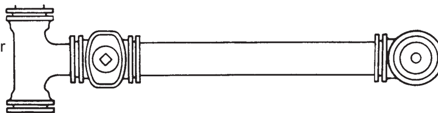
Typical installation perpendicular to the main using standard MJ tee, Coupling, MJ valve, Pipe, and MJ Hydrant.
