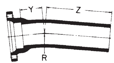
11 1/4° MJxPE (1/32)
