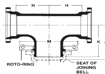
Anchoring Tee, Mechanical Joint
