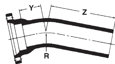
22 1/2° MJxPE (1/16)
