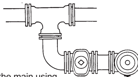
Typical installation perpendicular to the main using standard MJ tee, Coupling, MJ valve, Pipe, and MJ Hydrant.
